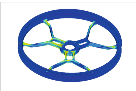
Stress contour plot of the wheel rim
